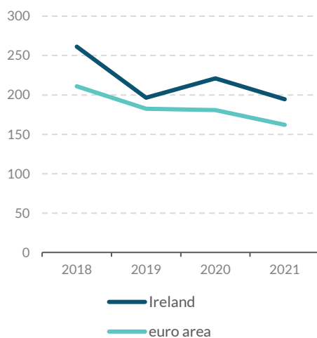
Figure 5 Tons of CO2 emissions per million euro
