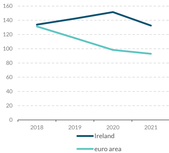
Figure 3 Tons of CO2 emissions per million euro
