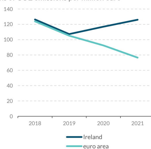
Figure 2 Tons of CO 2 emissions per million euro
