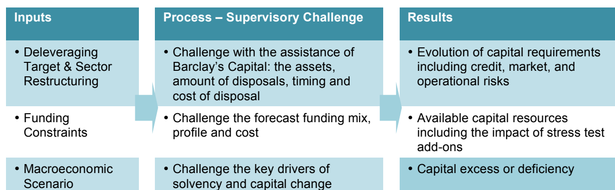
Figure 1: PCAR methodology
